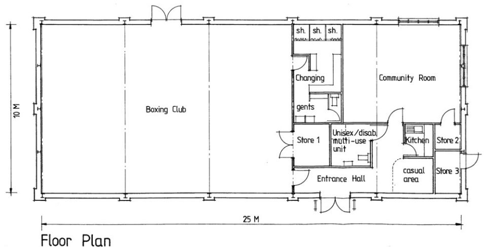
The floor plan for the new boxing club and community youth facility at Wheeler Road, Ludlow
